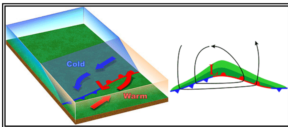
Figure 11-10. Wave Cyclone Model—Stage 2
