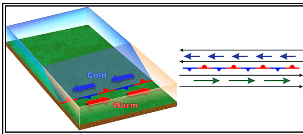
Figure 11-9. Wave Cyclone Model—Stage 1
