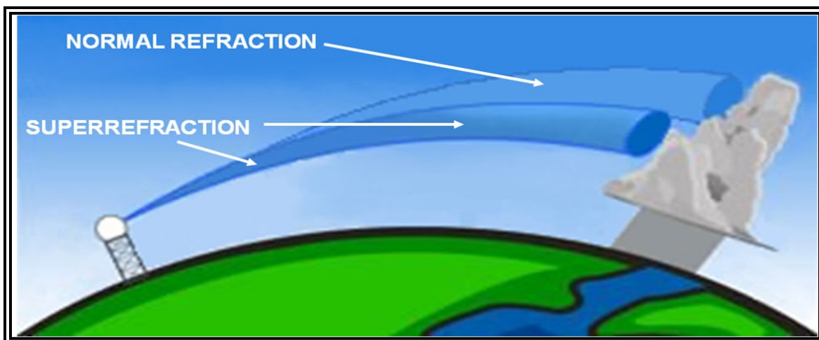
Figure 15-10. Superrefraction
